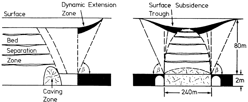
Figure 5. Wide Face at Shallow Depth.
