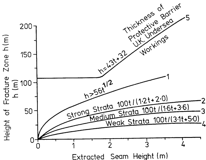
Figure 2 - Height of fracture zone ( h ) above a longwall face for various thicknesses of extraction, t (m).
