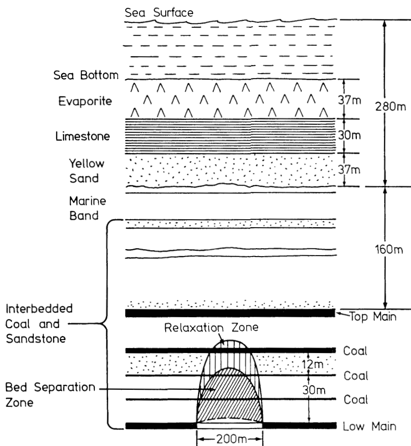
Figure 13. Under Sea Working at Great Depth.
