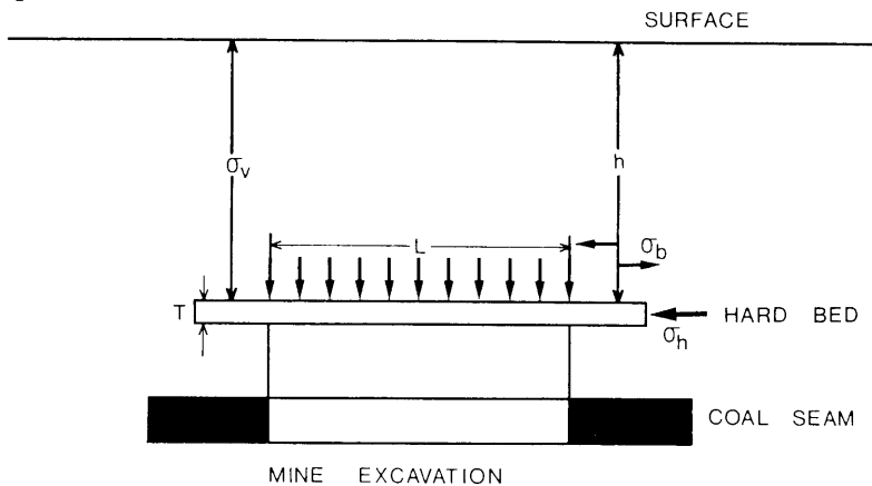
Figure 4. Theory of a Massive Bed Bridging over and Excavation.
