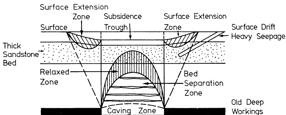
Figure 11. Shallow Headings Passing Through Hard Strata Connected to Surface Extension Zone.
