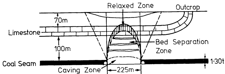
Figure 10. Bed Separation Zone Linked to a Jointed Limestone Bed Outcropping a Certain Distance Away.
