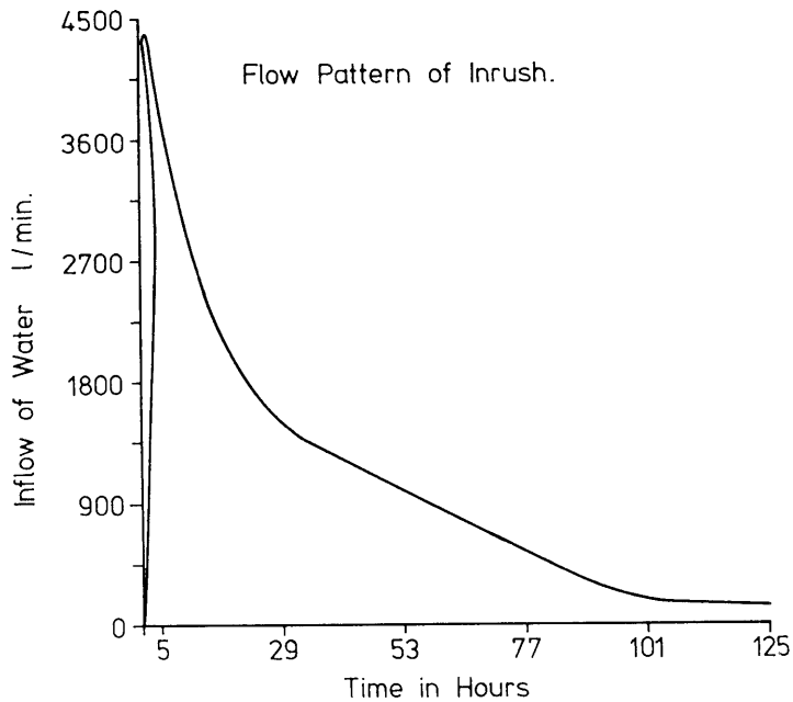
Figure 3 (b). Flow Pattern of Event Controlled Inundations, (Pugh 1981)
