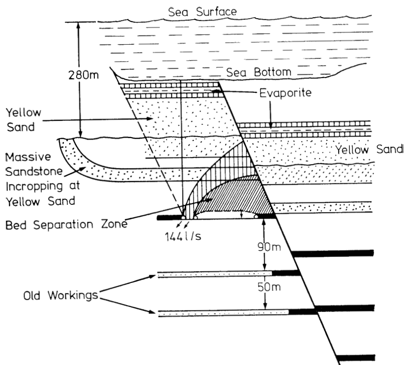
Figure 12. Under Sea Workings in Hard Stars in Faulted Zone.
