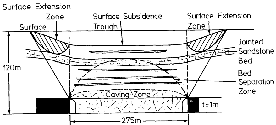
Figure 6. Shallow Caving Workings.
